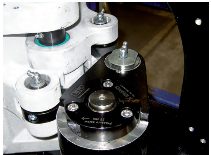
Lever fastened with ETP-EXPRESS to open/close the mold.
