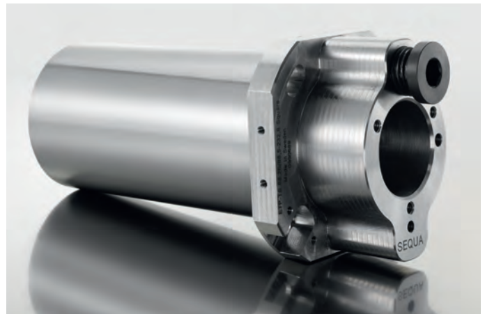
ETP-AXPRESS (a version of ETP-EXPRESS where the pressure setting is done in the axial direction). Decorator for 2 piece beverage cans.
