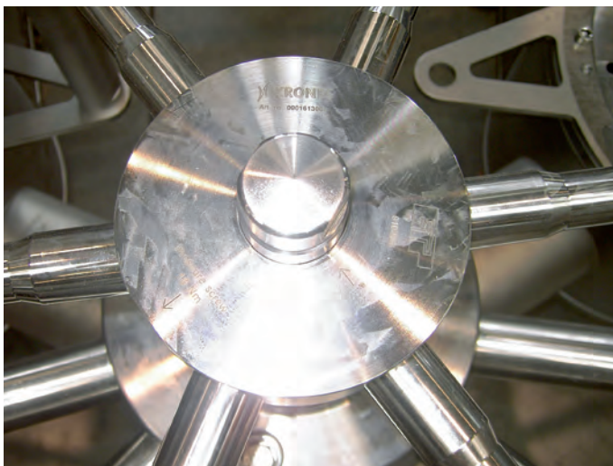
This ETP-EXPRESS R is made of high grade stainless steel, because it is washed regularly with an aggressive cleaning fluid.
