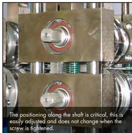
Rollers are easily changed using ETP-POWER and especially beneficial in high production applications.
