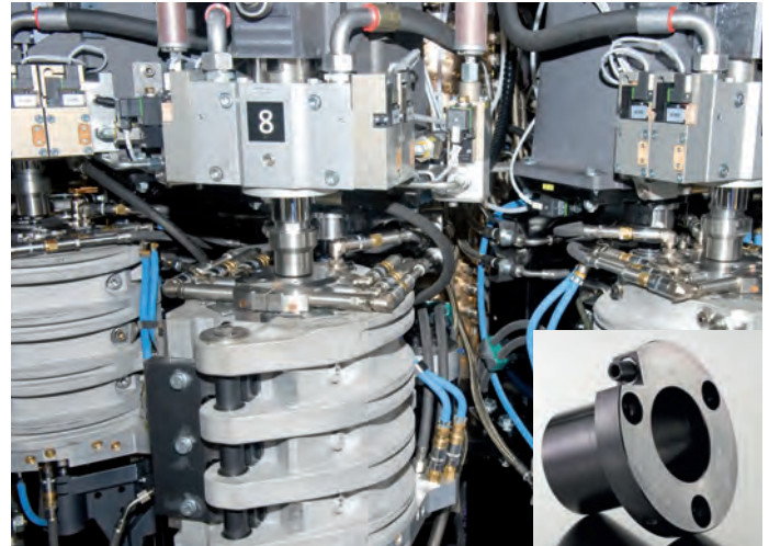
Complete blow mold unit with several molds/cavities.
