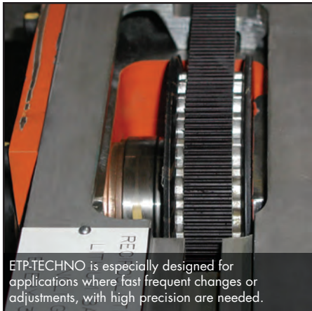
In a test rig for vehicle gearboxes the output shaft is connected to a torque limiter with ETP-TECHNO to control the torque transmission.
