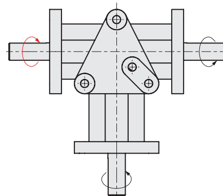
Counter-Rotating Crown
